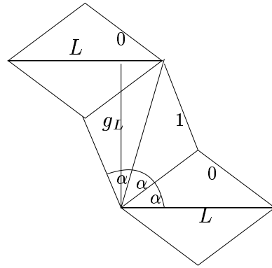
FIGURE 5. g_L is a simple periodic loop.
