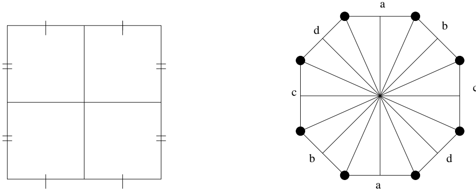
FIGURE 1. Invariant surfaces.
