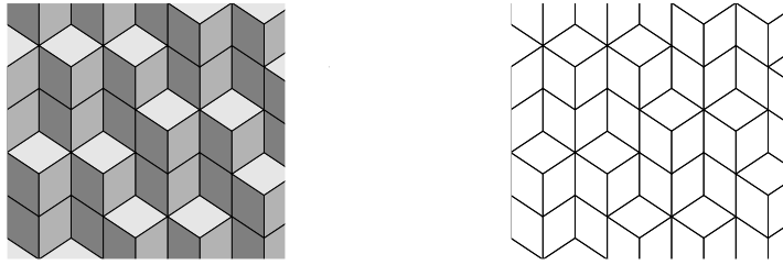
Figure 3. From a stepped plane to a tiling of the plane \Delta by three kind of lozenges.
