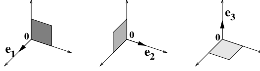
Figure 1. Examples of faces in \mathbb{R}^3 .
