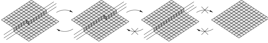
Figure 8. One can transform the first stepped surface into the second one, and conversely, by performing a finite number of flips. A locally finite sequence of flips allows one to transform the second stepped surface into the third one (we perform an infinite and locally finite sequence of flips which rejects to the infinity the only face of type 1*), but the converse transformation is impossible (no flip can be performed). Lastly, we can neither transform by flips the fourth stepped surface into the third one, nor conversely.
