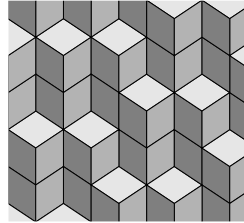
Figure 2. A piece of a stepped plane in \mathbb{R}^3 .
