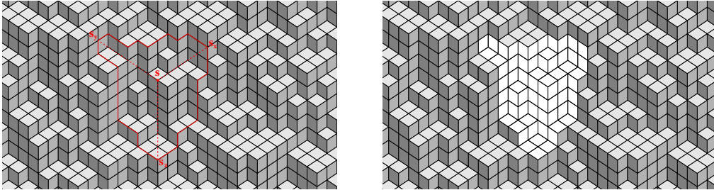
Figure 10. Given a stepped surface \mathfrak{S} , a vertex \mathbf{x} \in \mathfrak{S}' \cap \mathbb{Z}^3 defines a subset \mathcal{T}_{\mathbf{x}} of \mathfrak{S} . Left: the vertex \mathbf{x} and \mathbf{x}_3 , and the boundaries of \mathcal{T}_{\mathbf{x}} . Right: the faces of \mathcal{T}_{\mathbf{x}} (in white). To \mathcal{T}_{\mathbf{x}} corresponds a lozenge tiling of a bounded and simply connected domain of \mathbb{R}^2 .
